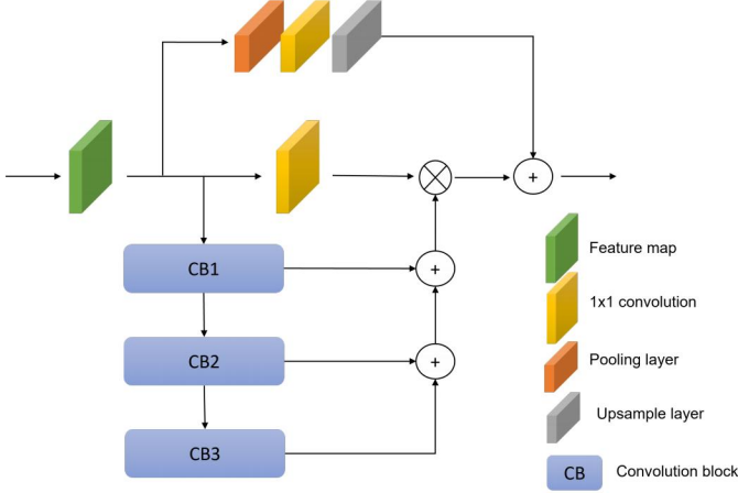
Fig. 3: Pyramid attention network architecture.
