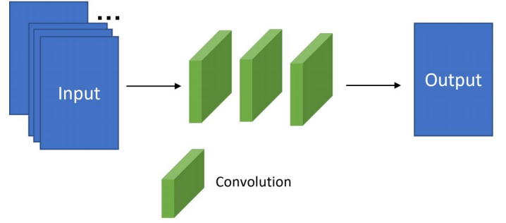
Fig. 5: Image reconstruction module architecture. There are three consecutive 3 \times 3 convolutional layers, each with the output channel 64, 32, and 1, respectively.
