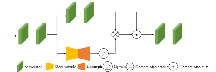
Fig. 2: Residual attention network architecture.
