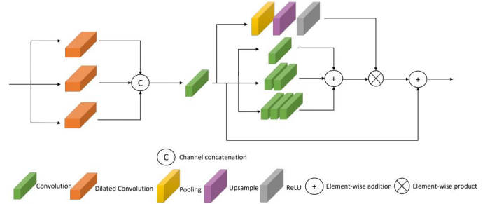
Fig. 4: Proposed Dilated Residual Attention Network architecture. Three pyramid convolution blocks contain one, two, and three consecutive 3 \times 3 convolutional layers, respectively.
