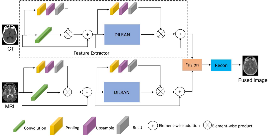
Fig. 1: The overall pipeline of the proposed method, which consists of a feature extractor, a fuser, and an image reconstructor
